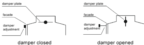
Fig. 5. The example of the damper adjustment
