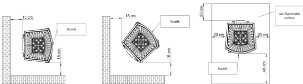
Fig. 2. Safe distances of the stove from non-flammable parts.
